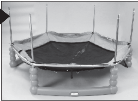
Layout trampoline mat with safety pad (A) flat. Place trampoline mat over assembled frame. Triangle rings should be underneath safety pad. Loop elastic on each corner over each of the straight frame tubes. Slide elastic down to the base as shown.
