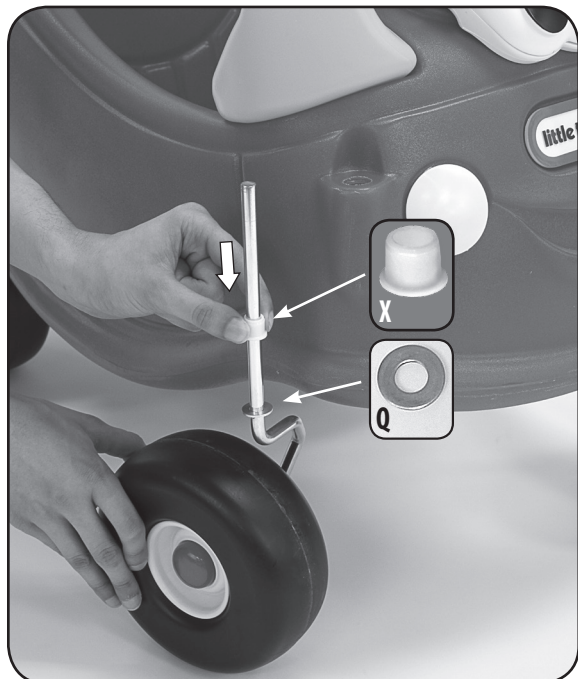
Slide washer, then bushing onto assembled right axle. Repeat on left axle.
