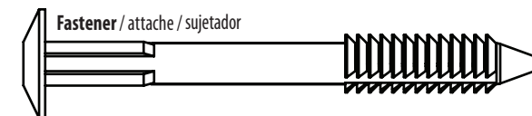
Person 1: hold down roof assembly. Person 2: install (2) fasteners (1 each side).
